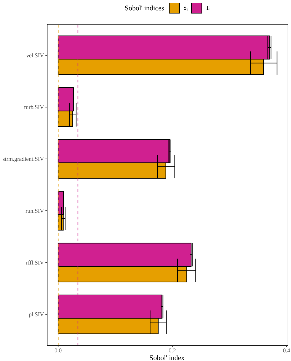
Figure 5. Results of a sensitivity analysis for the flatheadcatfishMacro model based on a geometric mean structure. Dashed lines represent baseline numerical approximation error for S_i and T_i ( i.e. , dummy variables).
